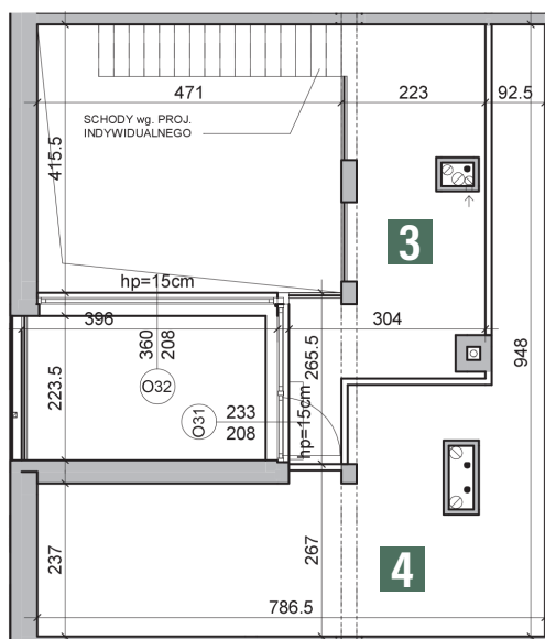
ANTRESOLA 13,33m 2
