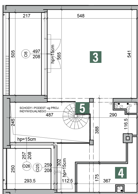
ANTRESOLA 43,08 m 2
