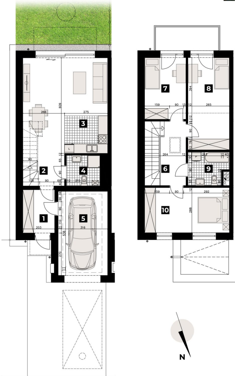
PARTER
